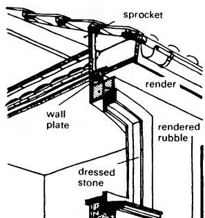
④ Rubble walls need framing with dressed stones → p. 37
